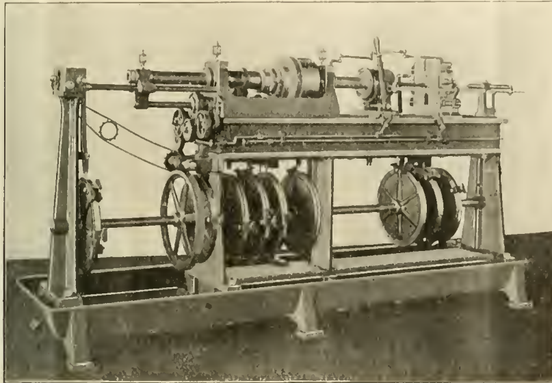
FRONT OF EPRIGHT'S AUTOMATIC STAYBOLT CUTTER.
